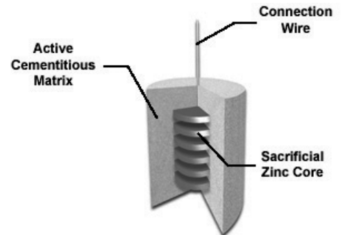
Cut-away of Sika Galvashield CC
